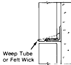
Weep Tube or Felt Wick Weep continuous and other angle supports where moisture collects.
