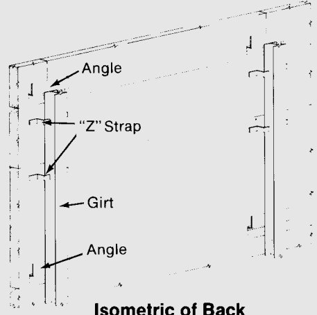
Isometric of Back of Typical Panels
