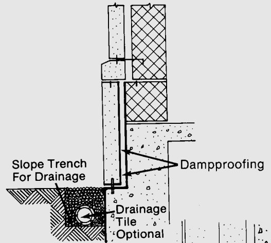
section b 2
