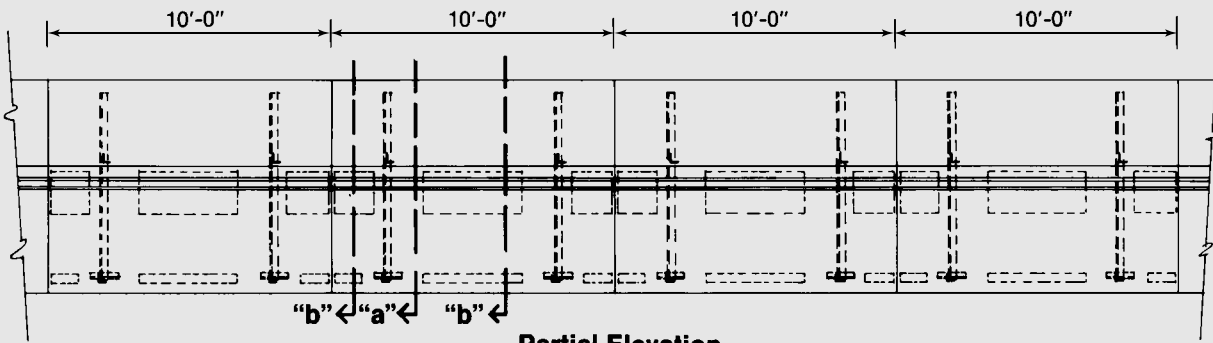
Partial Elevation
