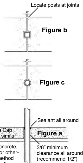
Typical Hand Rail Post Detail
