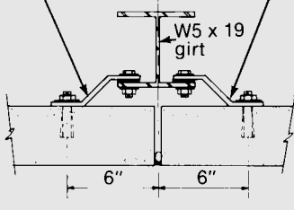
Plan Detail "B"
